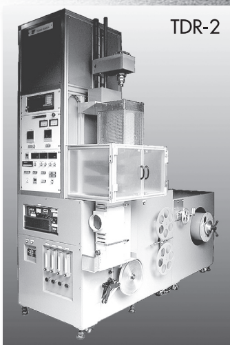
Optical Fiber Drawing System
